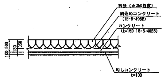
(石張水叩工補修)
