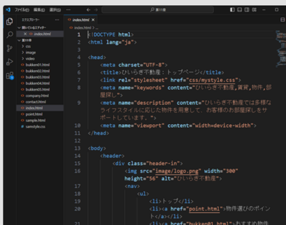
HTML・CSS
